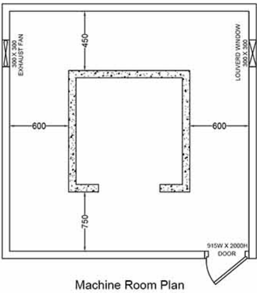
Passenger Lift With Manually Operated Doors – Geared Machine With Machine Room (Back Counter Weight)
