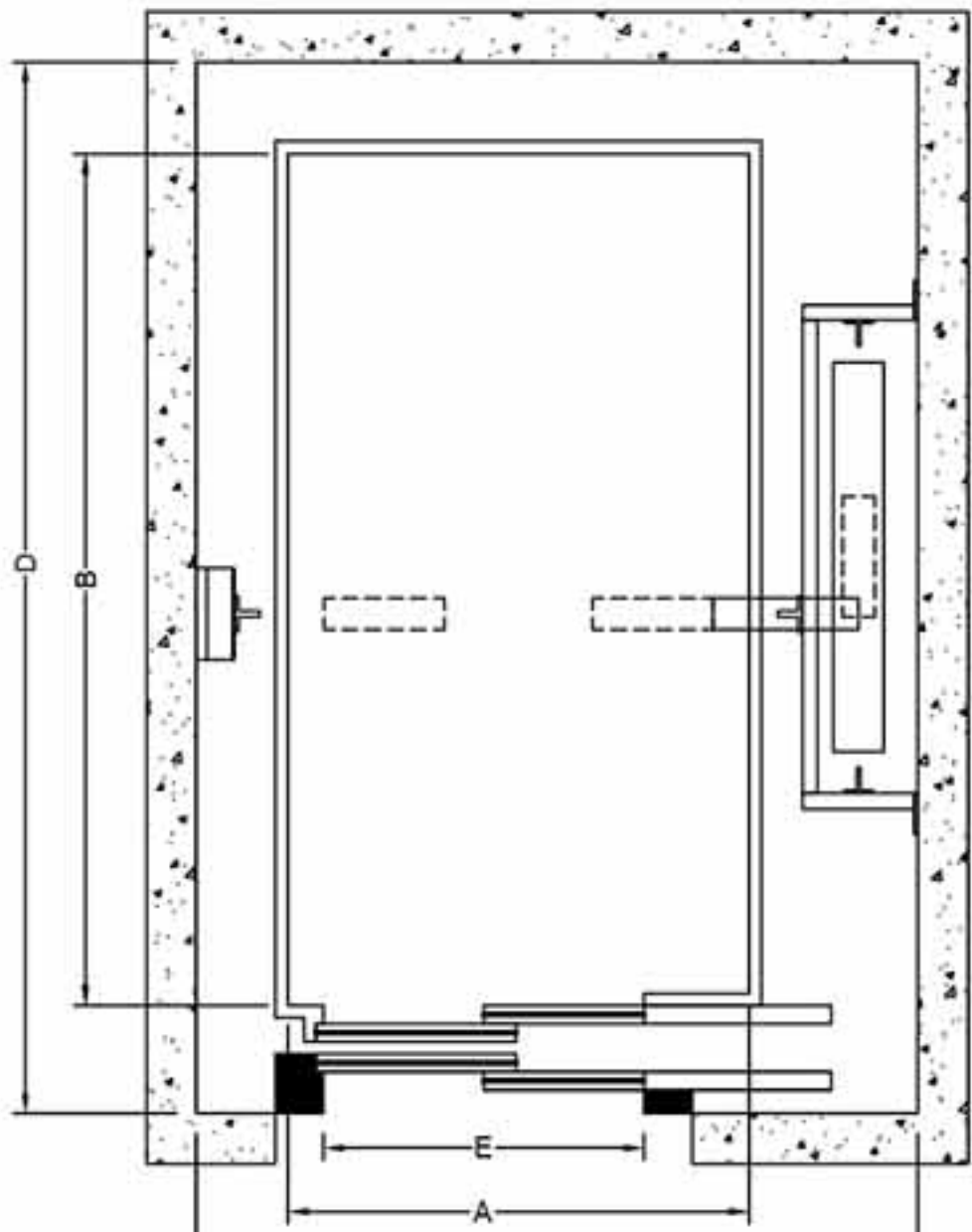
Hoistway Elevation & Plan For Telescopic Door. (Side Opening)
