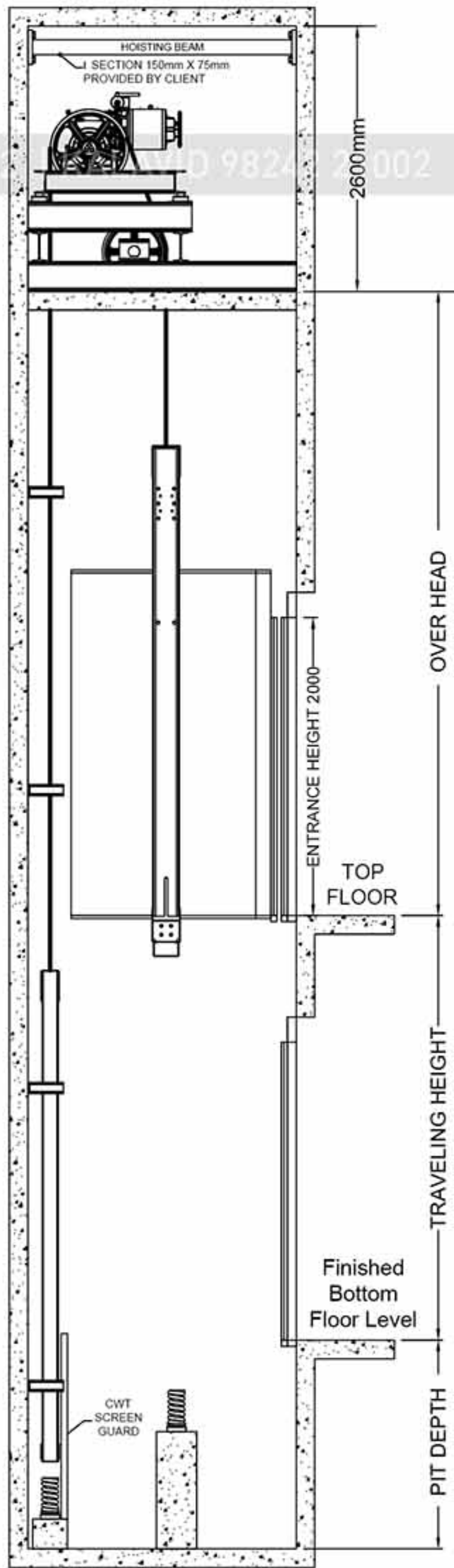
Hoistway Section View
