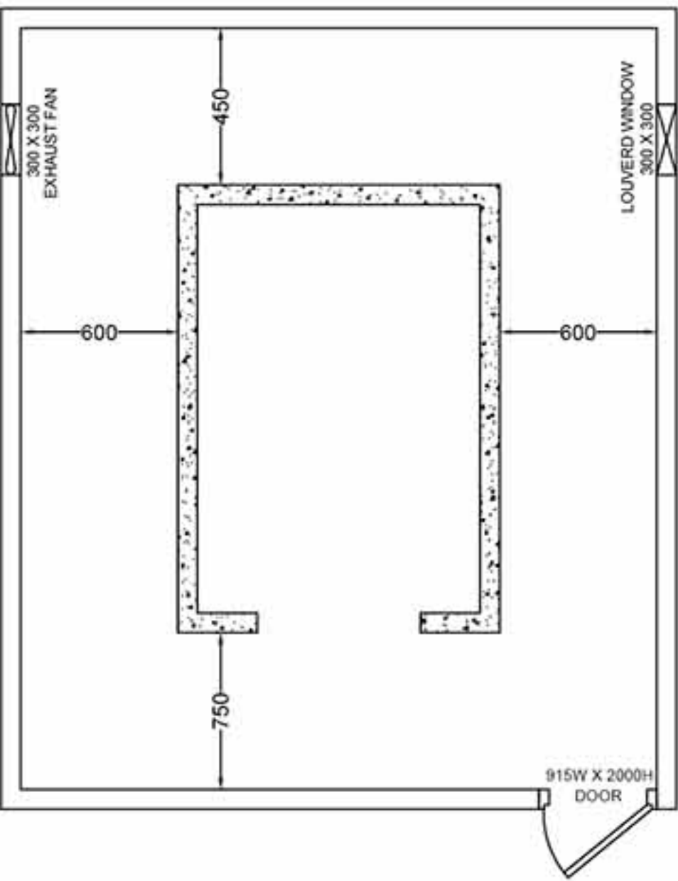
Machine Room Plan
