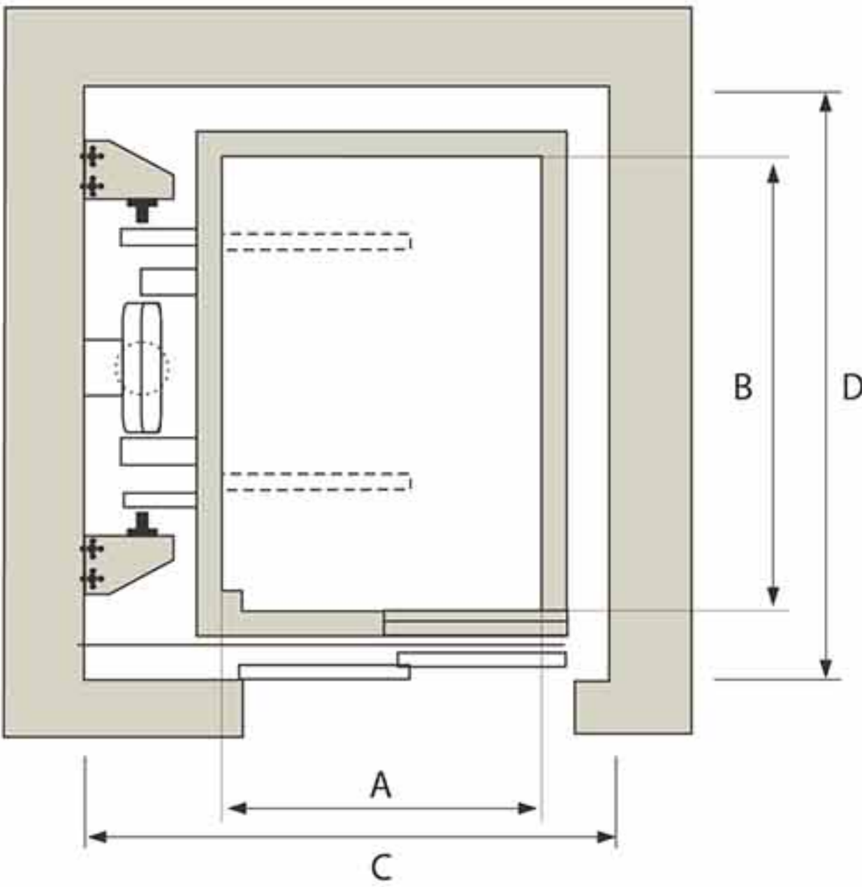
Hoistway Elevation & Plan
